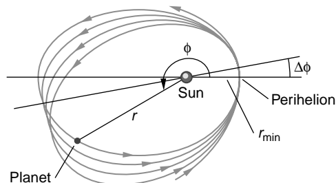
Fig. 2-21 The elliptical planetary orbits have the sun at one focus. The smaller gravitational forces due to the other planets cause the major axes to slowly rotate about the sun, shifting the line from the sun to the perihelion through an angle \Delta\phi each orbit. This shift is referred to as the precession of the perihelion. For Mercury, \Delta\phi = 9.55 arc minutes per century.
