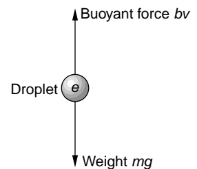
Fig. 3-5 An oil droplet in the cloud carrying an ion of charge e falling at terminal speed, i.e., mg = bv .
