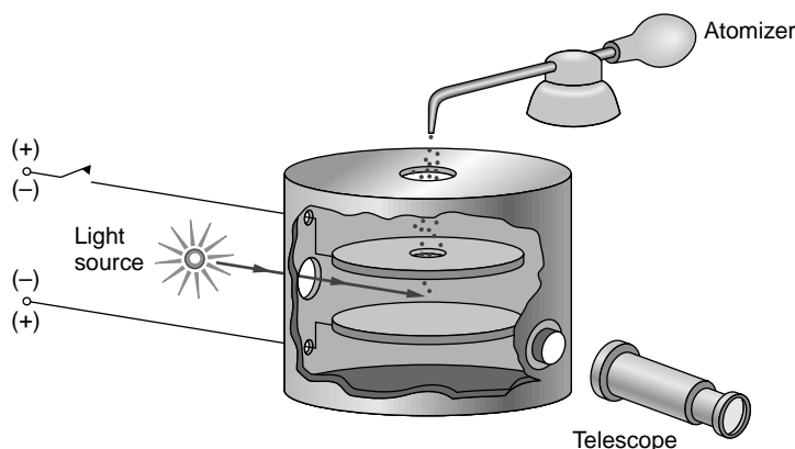
Fig. 3-4 Schematic diagram of the Millikan oil-drop apparatus. The drops are sprayed from the atomizer and pick up a static charge, a few falling through the hole in the top plate. Their fall due to gravity and their rise due to the electric field between the capacitor plates can be observed with the telescope. From measurements of the rise and fall times, the electric charge on a drop can be calculated. The charge on a drop could be changed by exposure to x rays from a source (not shown) mounted opposite the light source.
